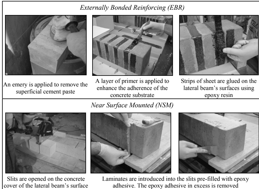
Figure 2 — Techniques for the shear strengthening of reinforced concrete beams
