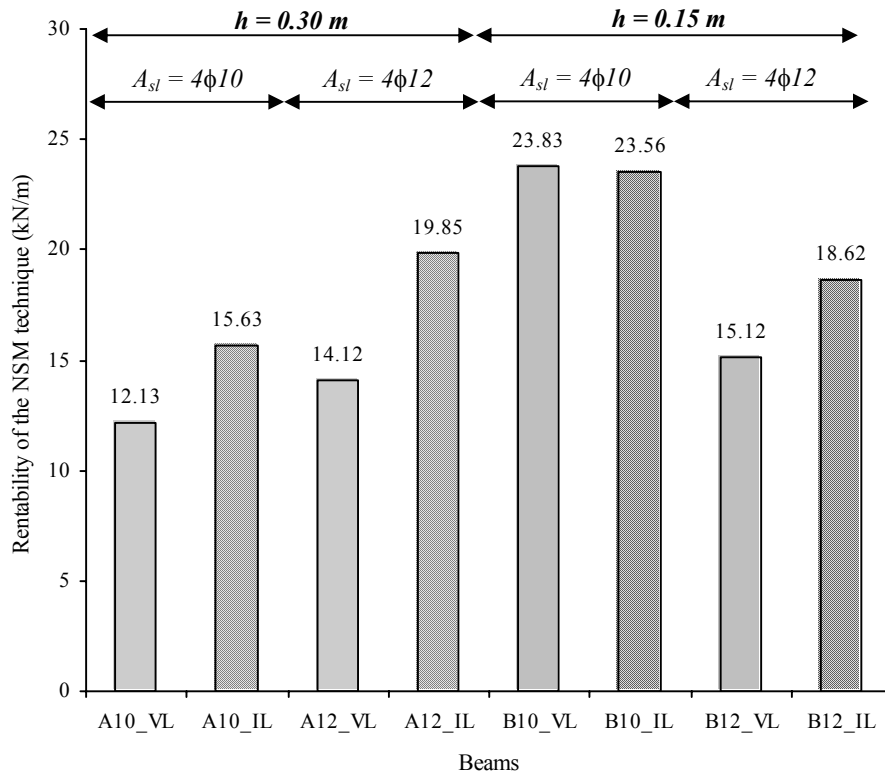
Figure 8 — Representation of the profitability index for the NSM technique
