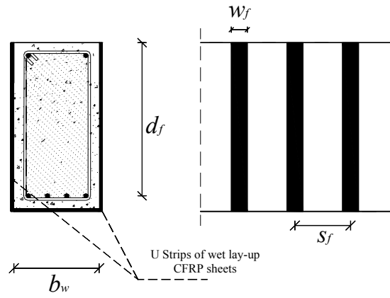
Figure 4 – Data for the externally bonded shear strengthening technique
