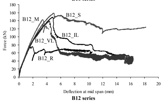
Figure 3 — Force-deflection relationship of the four tested beams series
