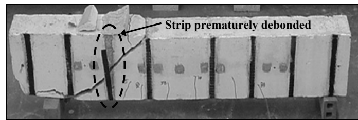
Figure 5 – Failure of A10_M beam
