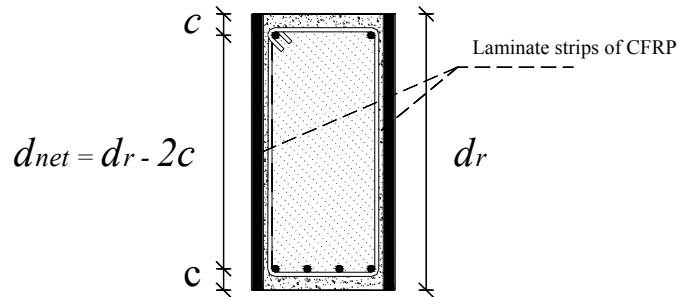
Figure 7 — Data for the near surface mounted shear strengthening technique
