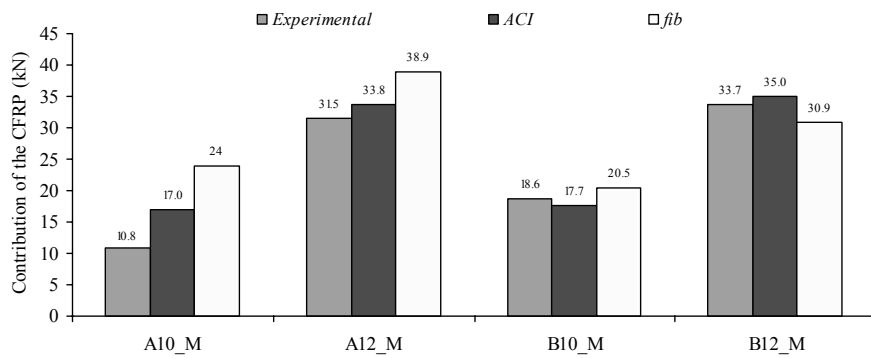
Figure 6 – Analytical vs experimental results (ACI and fib analytical formulation)
