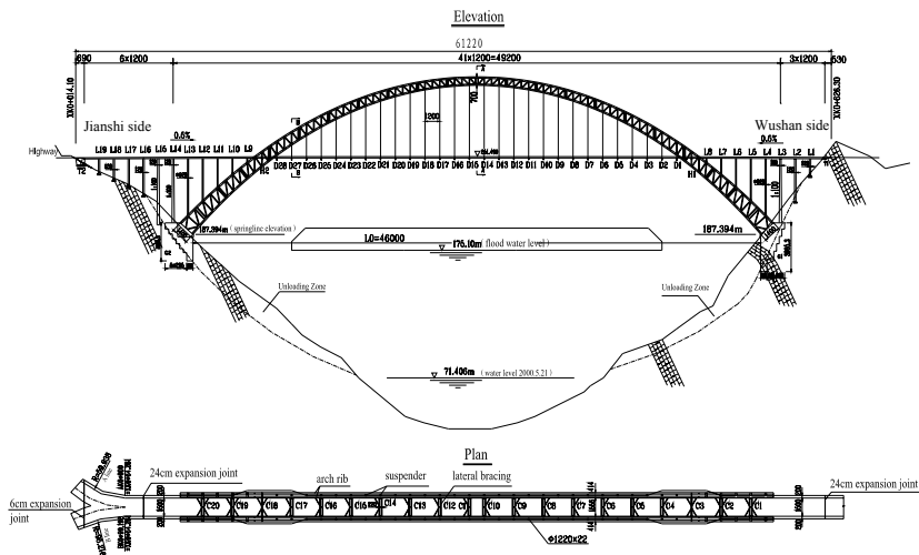
Figure 1: General plan of Wuxia Yangtze River bridge
