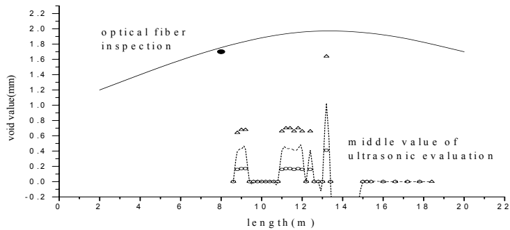
Figure 7: Arch crown void distribution of 6# tube
