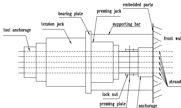
Figure 4: Layout of tension end of low stress anchorage system
