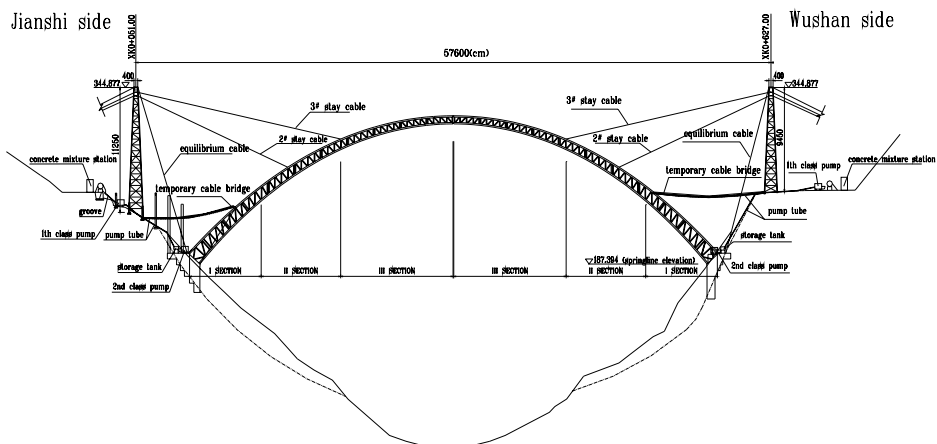
Figure 6: Layout of pouring concrete filled in tube
