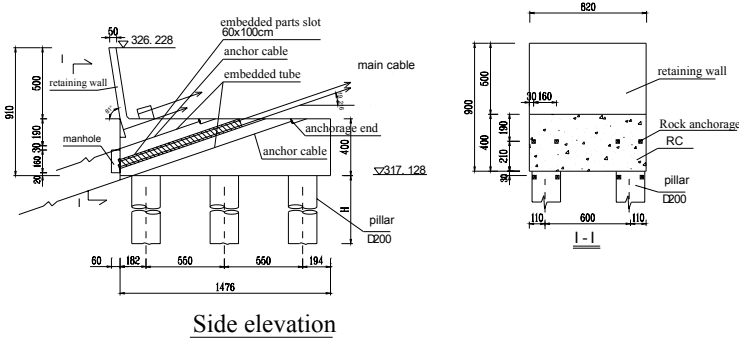
Figure 3: Layout of hoisting anchorage
