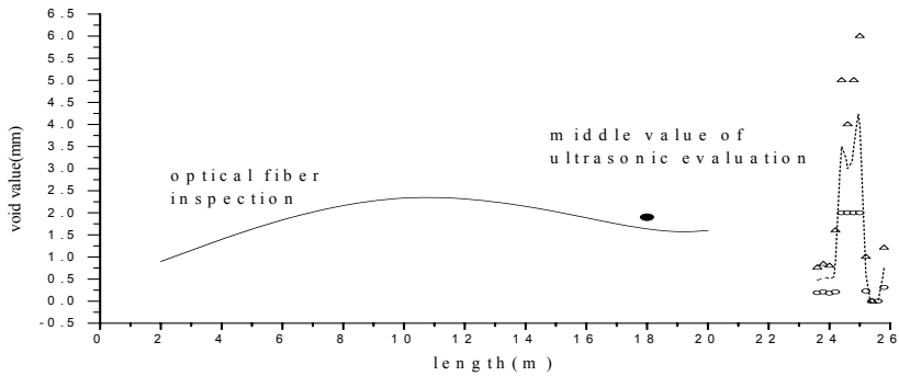
Figure 8: Arch crown void distribution of 8# tube
